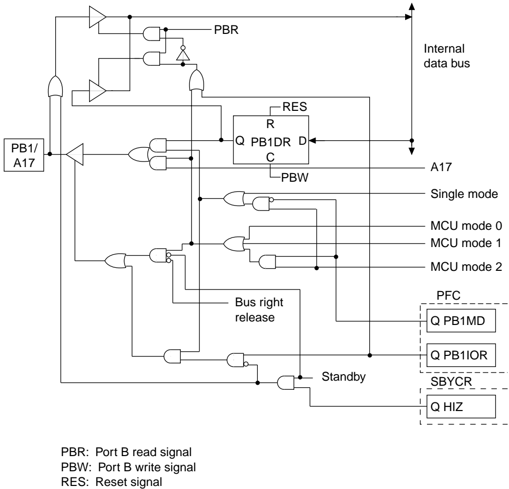
Figure B.16 PB1/A17 Block Diagram
