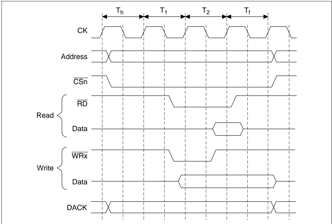
Figure 10.6 \overline{CS} Assert Period Extension Function
