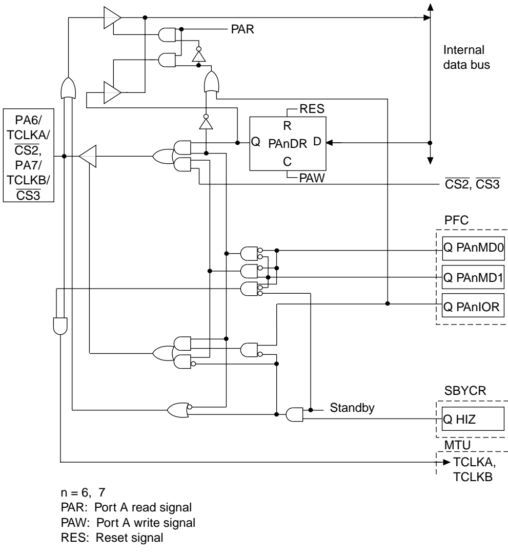
Figure B.3 PA6/TCLKA/CS2, PA7/TCLKB/CS3 (ZTAT, Mask) Block Diagram
