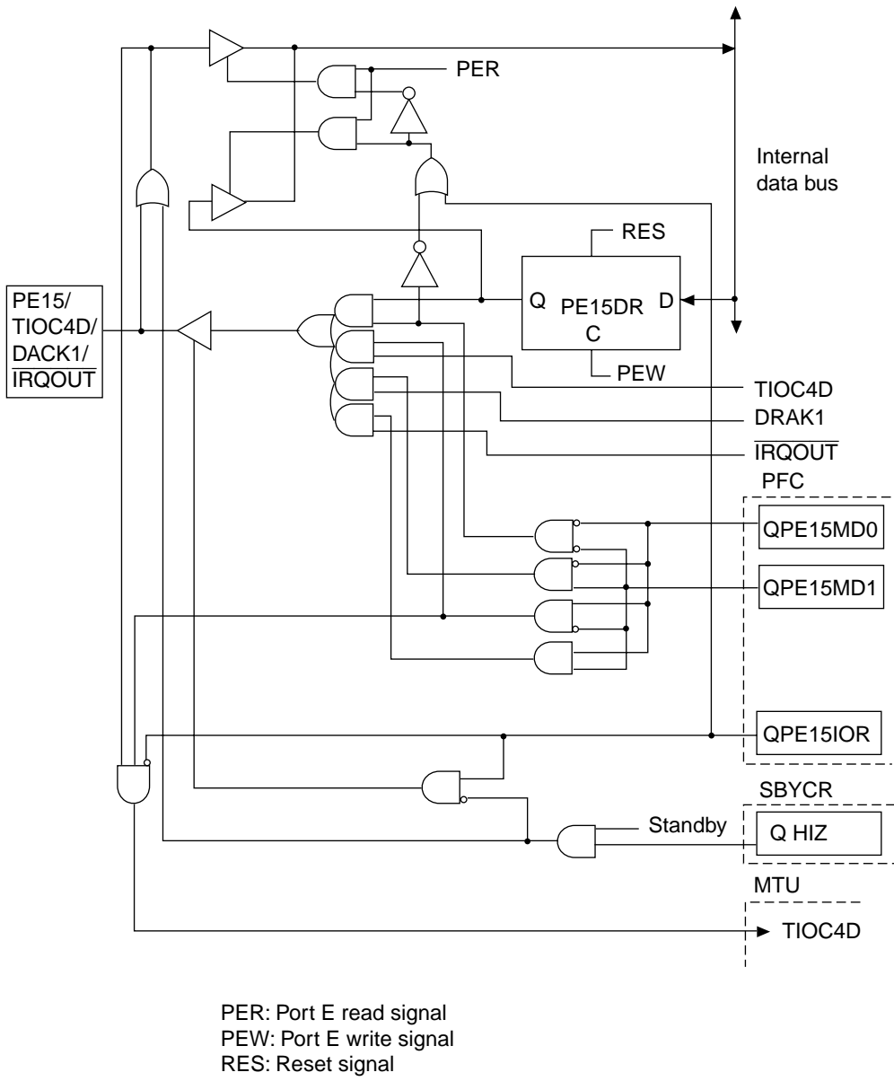
Figure B.35 PEn/TIOC4D/DACK1/IRQOUT Block Diagram
