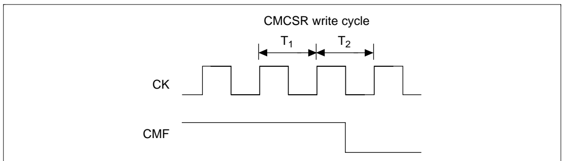
Figure 17.5 Timing of CMF Clear by the CPU
