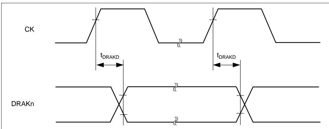
Figure 26.22 DRAKn Output Delay Time
