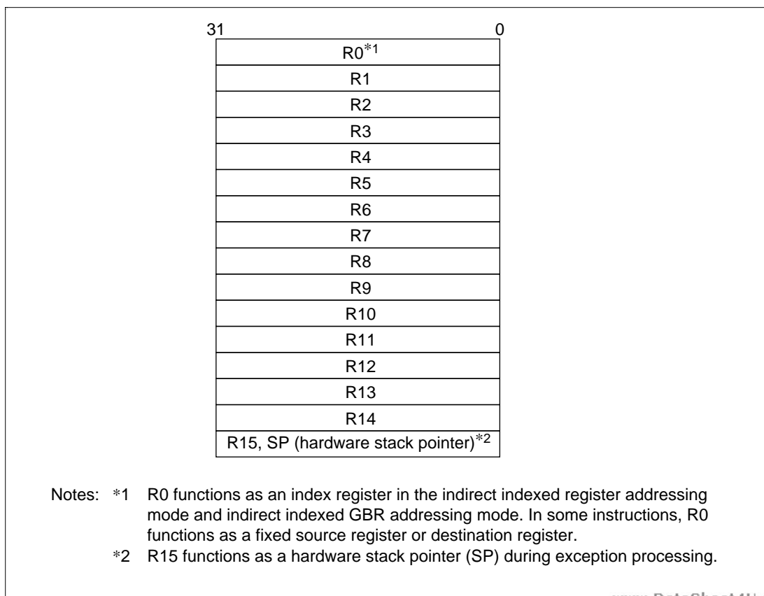
Figure 2.1 General Registers
