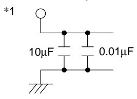
Figure 15.14 Example of a Protection Circuit for the Analog Input Pins
