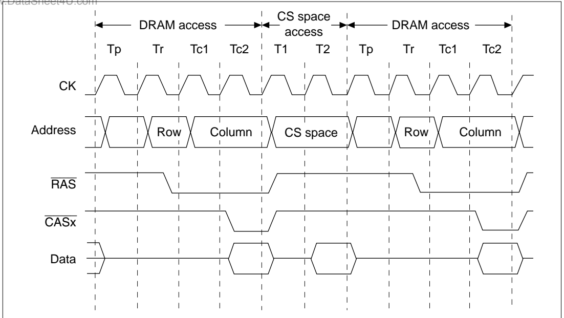
Figure 10.13 DRAM Access Normal Operation (RAS Up Mode)
