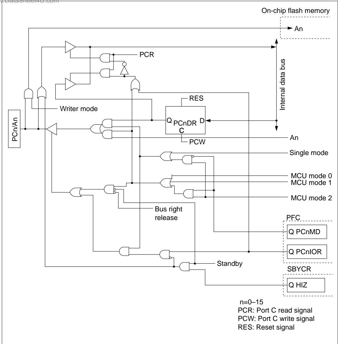
Figure B.23 PCn/An Block Diagram (F-ZTAT Version)
