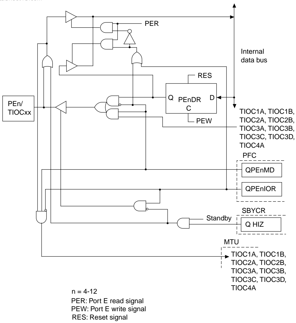
Figure B.36 PEEn/TIOcXX Block Diagram
