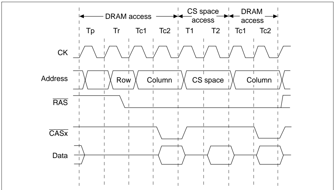
Figure 10.14 RAS Down Mode
